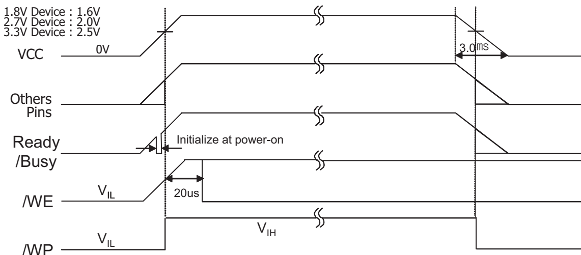
Figure 28: Power-on/off sequence
